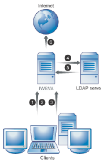
FIGURE 7-1. LDAP Communication Flow Using Kerberos Authentication
