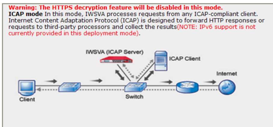
FIGURE 2-6. ICAP Mode
