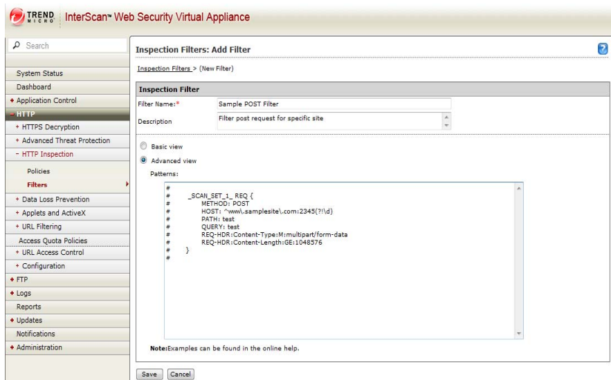
FIGURE 8-4. Sample Request mode POST filter in Advanced view
