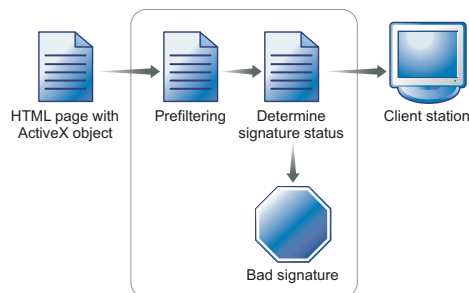
FIGURE 8-18. How ActiveX Security Works
