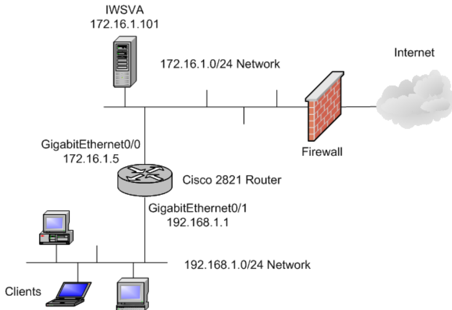
FIGURE F-1. Example Topology for Cisco 2821 Router Implementation
