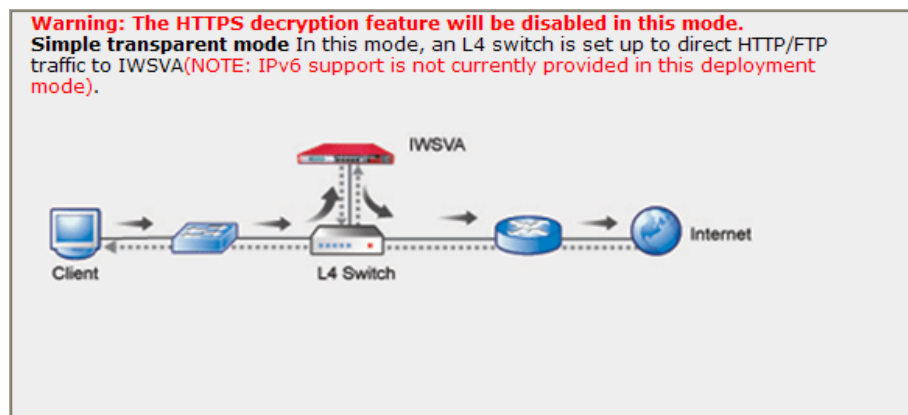
FIGURE 2-7. Simple Transparency Mode
