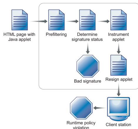
FIGURE 8-17. How Java applet security works
