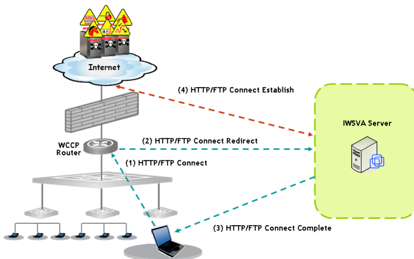
FIGURE 6-1. WCCP configuration and Web and FTP traffic
