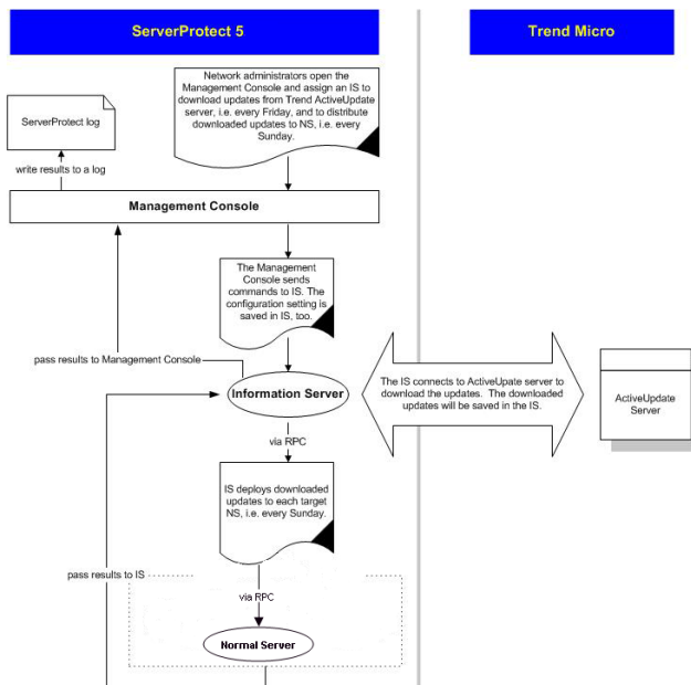
FIGURE 3-38. How Updates Work
