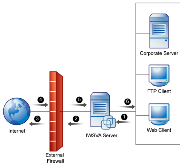
FIGURE 2-2. One Firewall with DMZ
