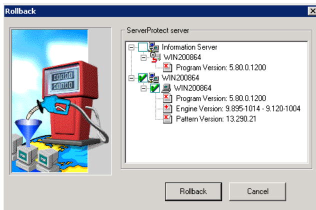
FIGURE 3-14. Rollback dialog
