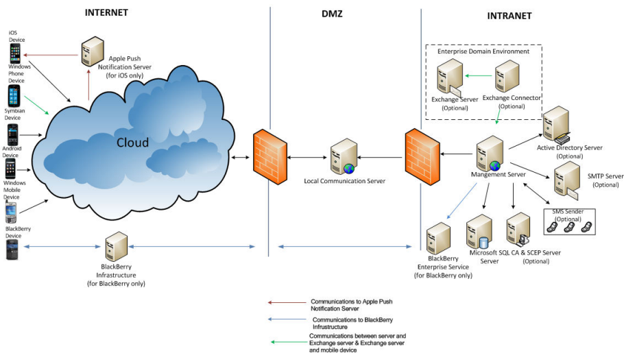
FIGURE 1-2. Enhanced Security Model with Local Communication Server
