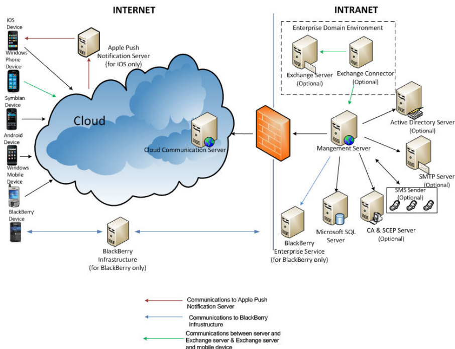
FIGURE 1-1. Enhanced Security Model with Cloud Communication Server
