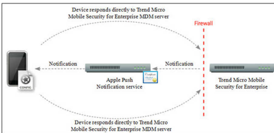
FIGURE C-1. Notification process
