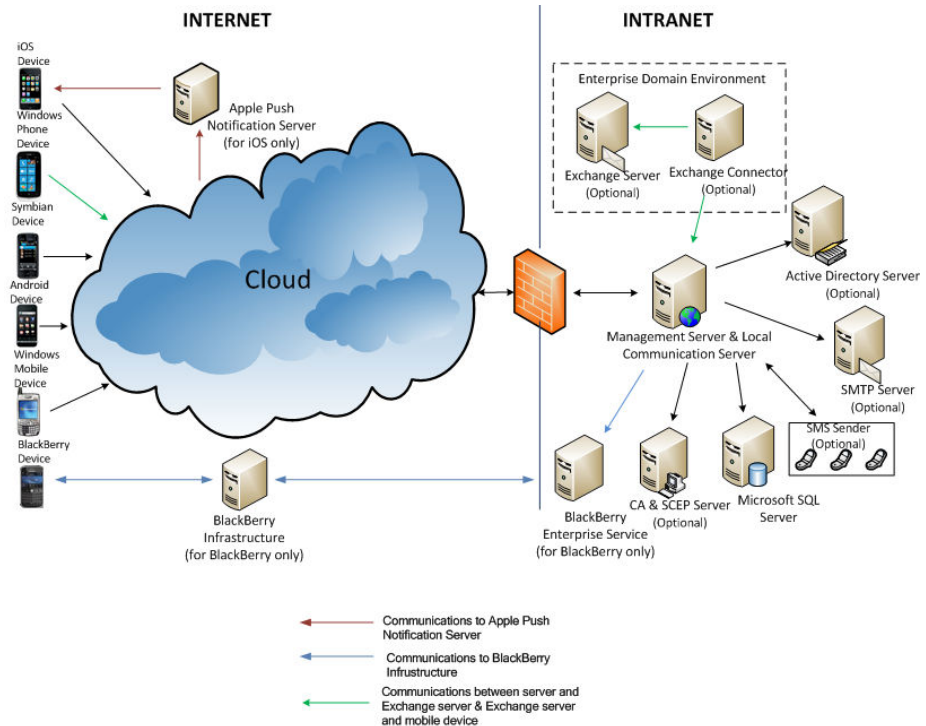
FIGURE 1-3. Basic Security Model
