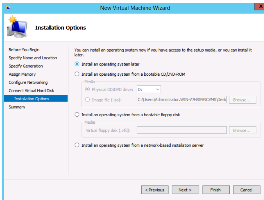
FIGURE C-12. Installation Options
