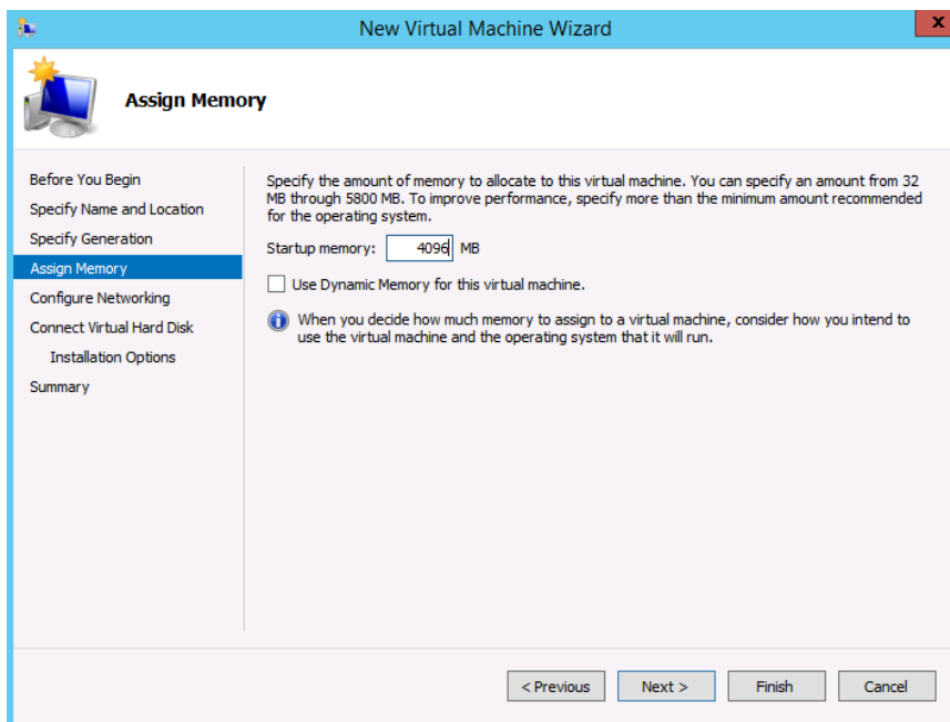
FIGURE C-9. Assign Memory
