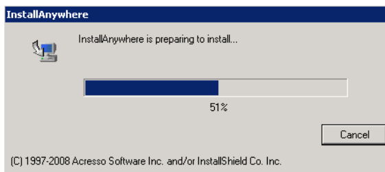
FIGURE 2-32. InstallAnywhere screen
